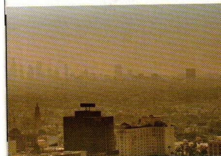
What causes smog? (Chapter 13)
